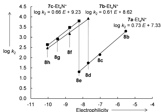
Figure 3. Correlation of the logarithm of the second-order rate constants k_2 for the reactions of triarylborohydrides 7c -NEt 4 + (■), 7b -NEt 4 + (▲), and 7a -NEt 4 + (●) with the benzhydrylium tetrafluoroborates 8b–h in MeCN at 20 °C with the electrophilicity parameters E of 8b–h from Table 1. [3]
